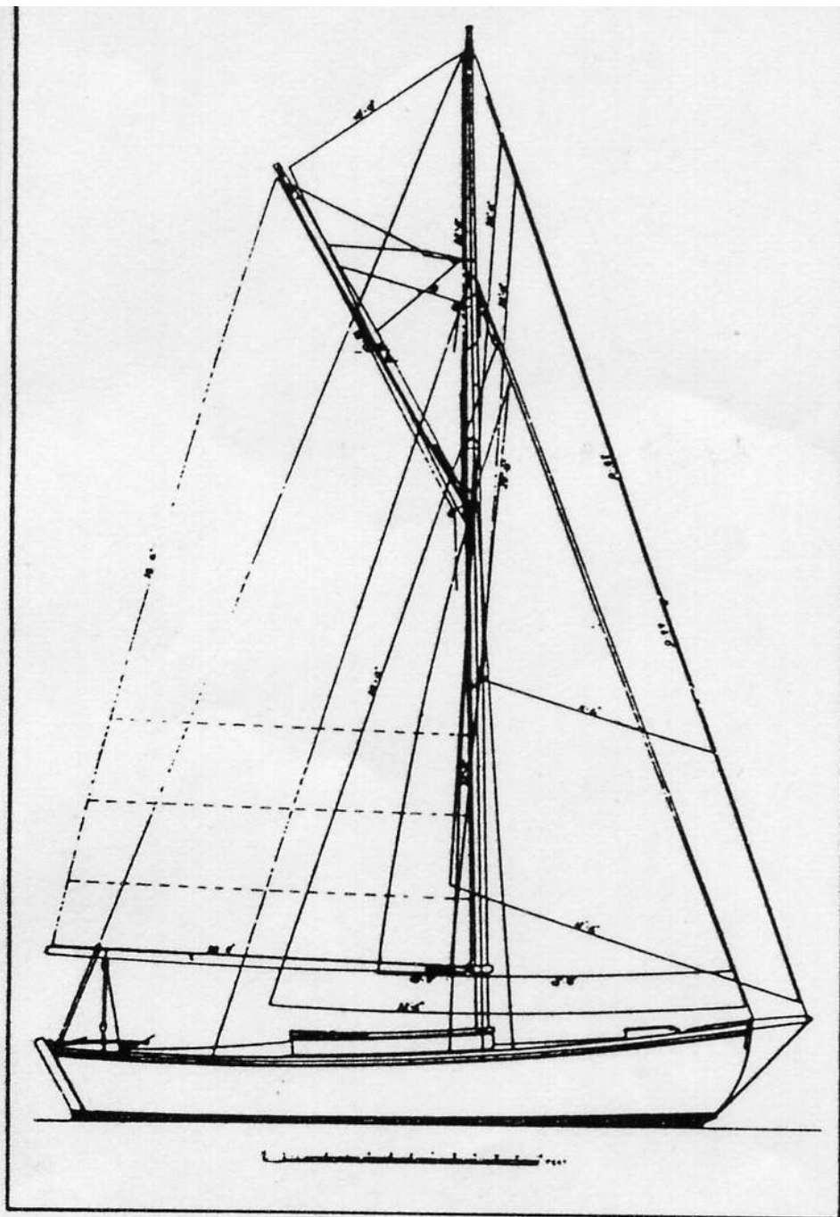
Racing sail plan of the fast cruiser Wanda, 1938. A Sandeman Quayside type successful in offshore racing.
